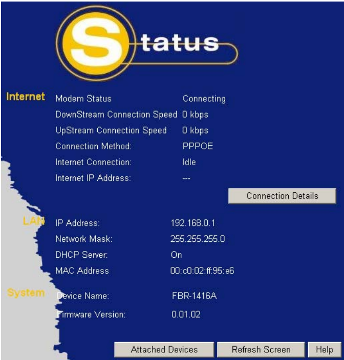
Figure 22: Status Screen
